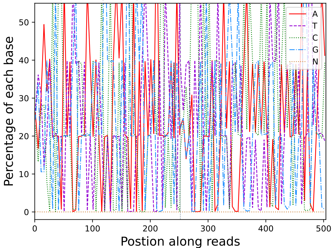
Base percentage along reads (R10905)
